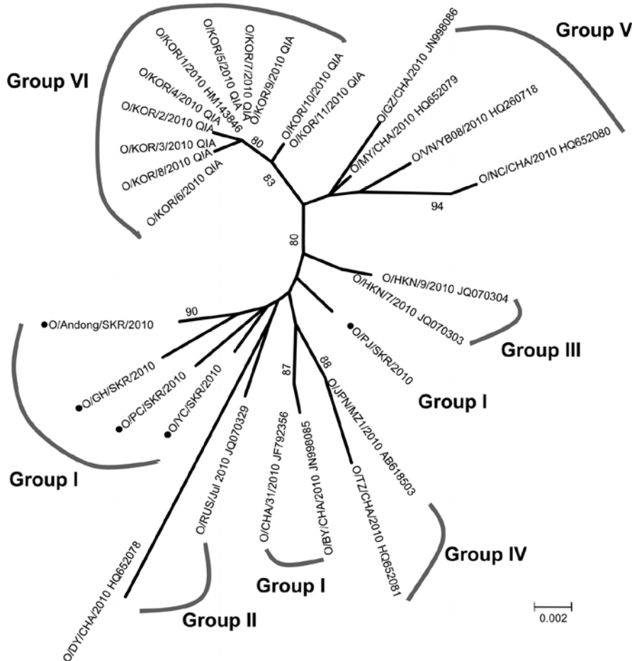
Figure 2. Phylogenetic analysis of viral protein 1 sequences of serotype O foot-and-mouth disease viruses isolated in South Korea (black dots) and other Asian countries, 2010. The tree was constructed by using the neighbor-joining method in MEGA5 ( www.megasoftware.net ). Percentages in which the associated taxa clustered together in the bootstrap test (1,000 replicates) are shown next to the branches. Scale bar indicates nucleotide substitutions per site. CHA, China; HKN, Hong Kong; JPN, Japan; RUS, Russia; SKR or KOR, South Korea; VN, Vietnam.
