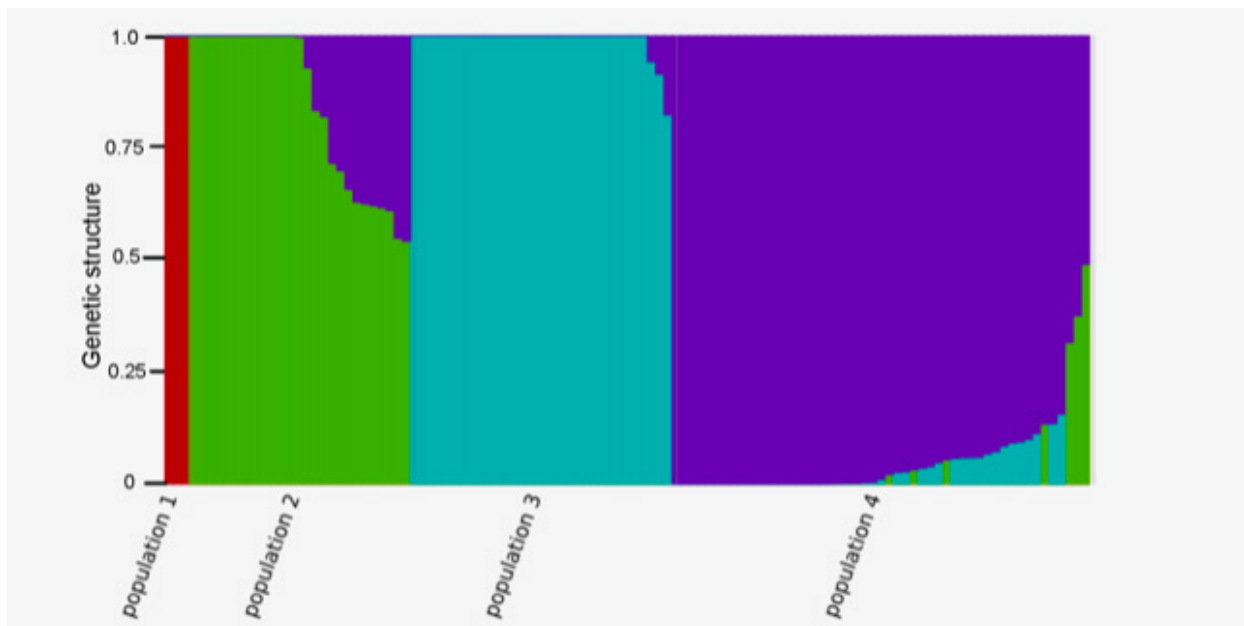
Appendix Figure. Population structure analysis of Blastomyces dermatitidis fungi based on 97,403 SNPs genotype calls across 108 strains. Each vertical line represents a strain and each color a separate population.
